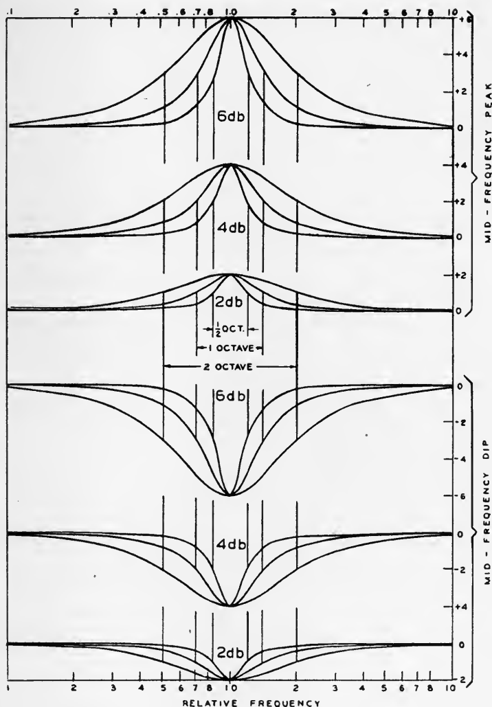
FIG. 2. Generalized relative response of equalizer sections which raise or lower a limited portion of the spectrum.
